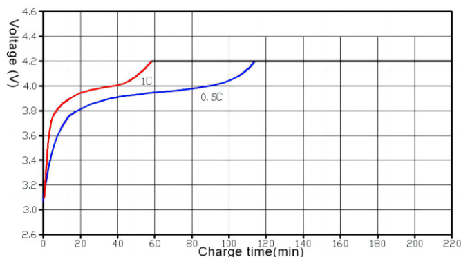
Different Rate Charge Curve
